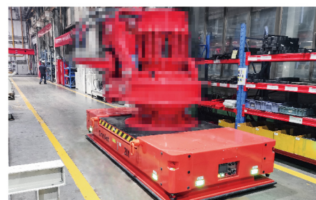
OmniAnt-动力头运输AGV(20t)
